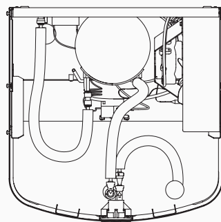
Top View of an Acorn Water Cooler - 27 Parts
